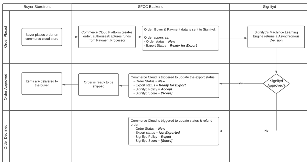
SFCC Post-Auth Flow
